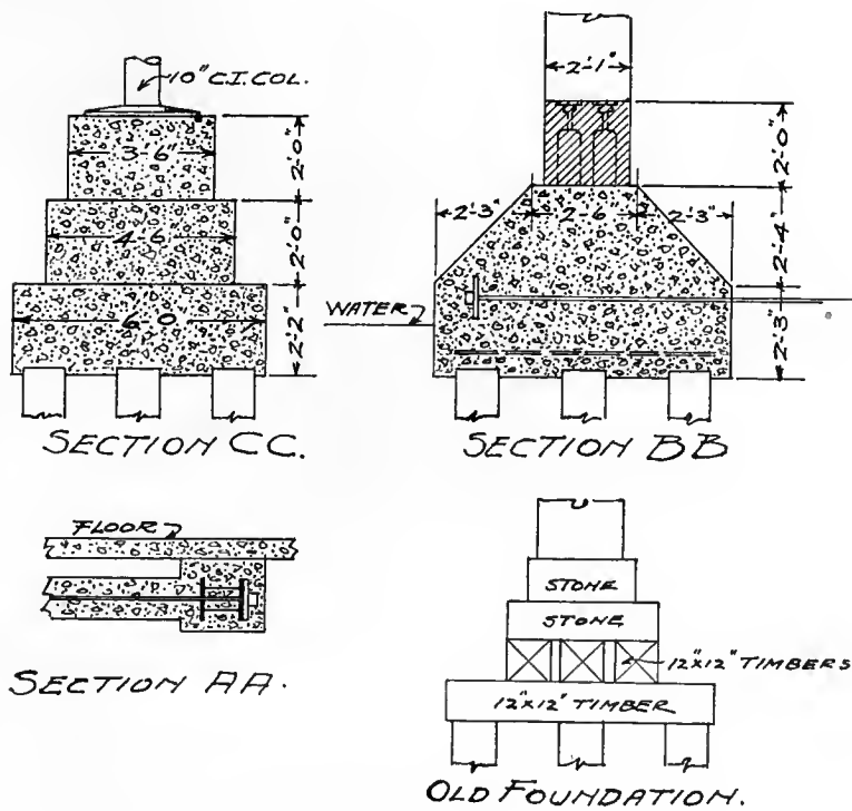
SECTIONS
